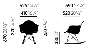
Eames Plastic Armchair RAR, Schommelstoel
